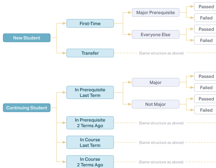
FIGURE 5 ➤ Flowchart Structure for the Conditional Probability Analysis
