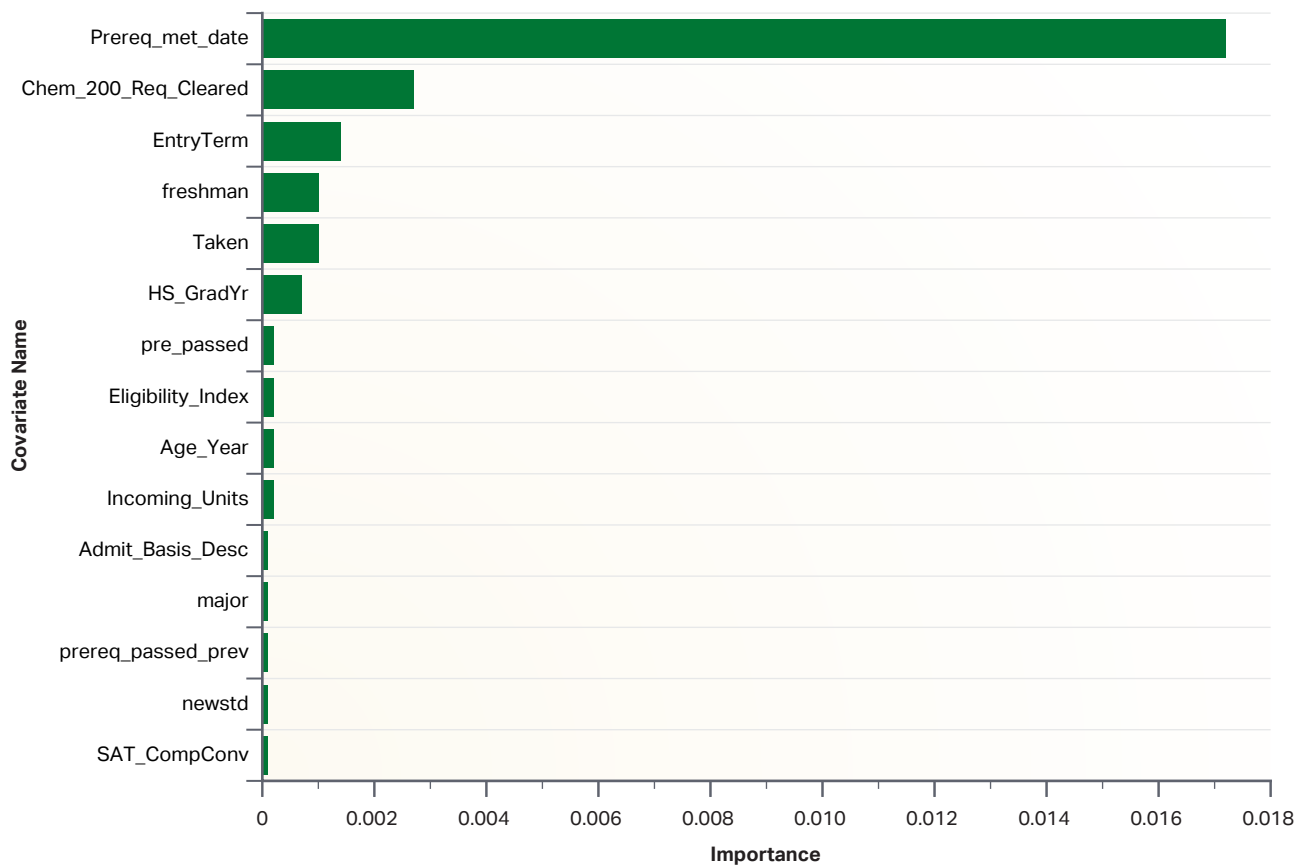
FIGURE 3 ► Variable Importance for Random Forest Application
