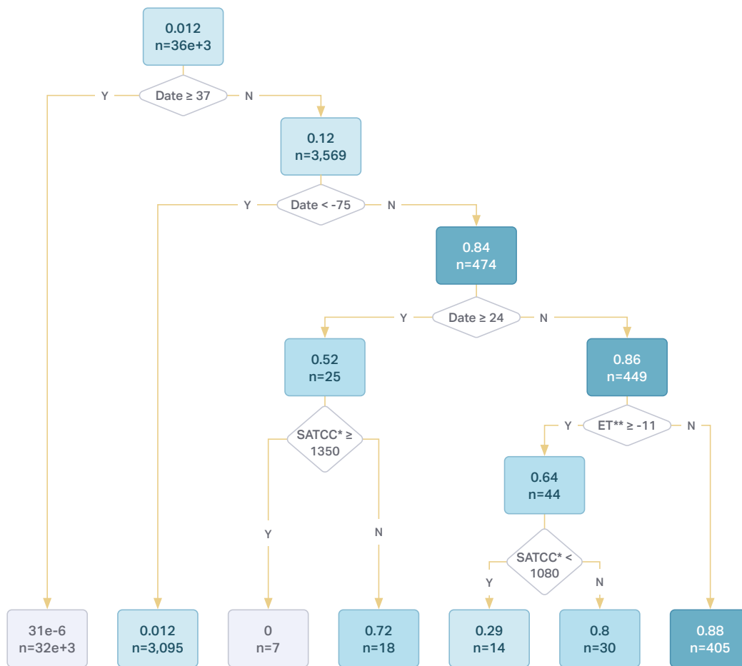
FIGURE 1 ► Classification Tree Analysis: Decision Tree Trained From 2017 Data
