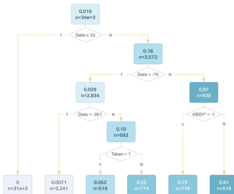
FIGURE 6 ➤ Classification Tree Analysis: Tree Trained Using 2015 Data
