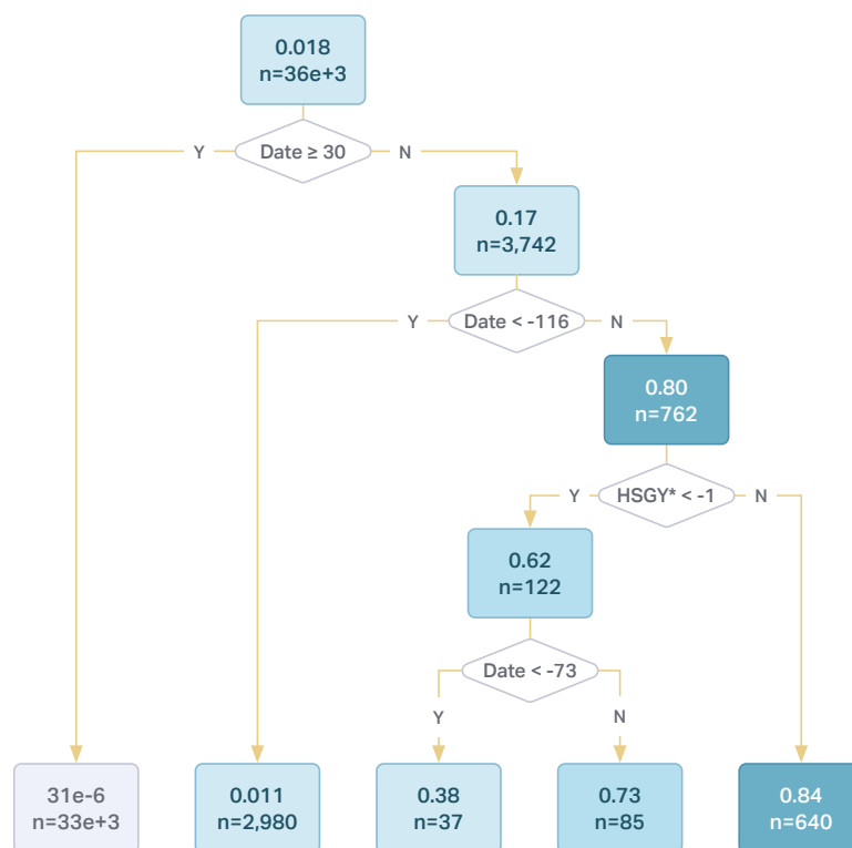
FIGURE 2 ► Decision Tree Trained from 2018 Data
